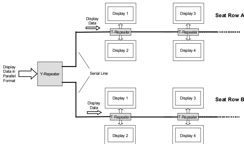
Figure 13 : Passenger Information System with GigaSTaR Line- and Y-Repeater
