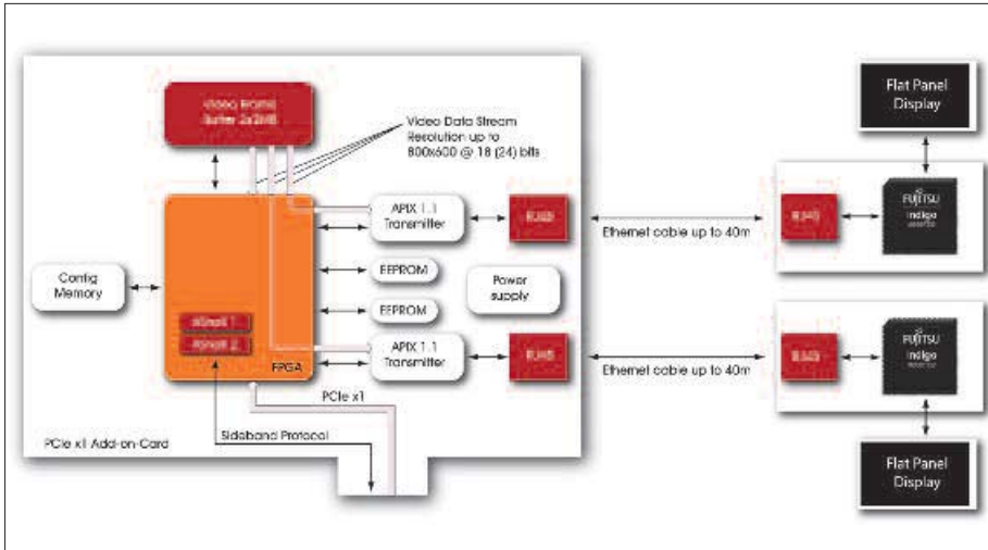
Figure 4: APIX 1.1. interface card block diagram (FPGA with PCIe core)
